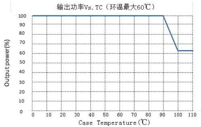
Output power VS Shell temperatur
