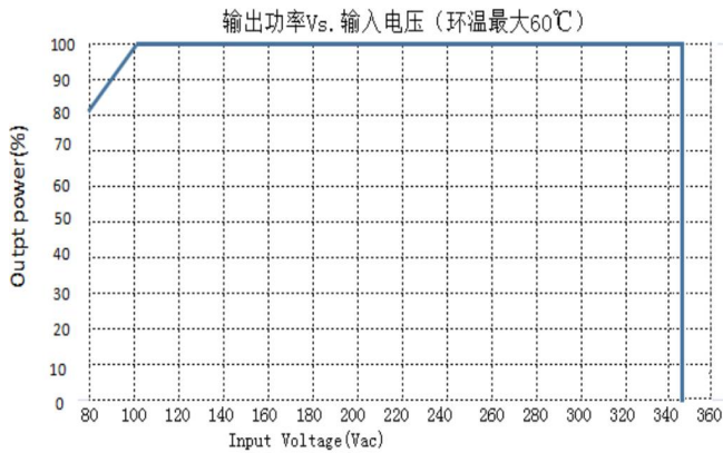
Output power VS Input voltag(50°C max.)
