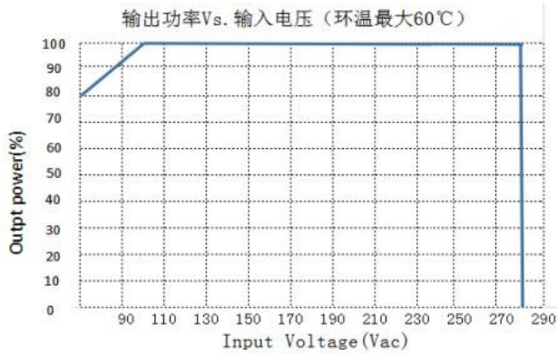
Output power VS Input voltg(50°C max.)
